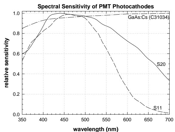
Fig. 2 Normalized spectral response of the sensitivity of the photocathodes used. See also Tab. II.
