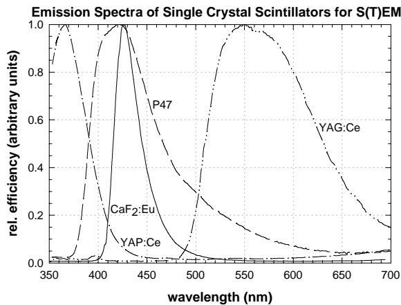
Fig. 1 Normalized cathodoluminescent spectra of single crystal scintillators for S(T)EM.
